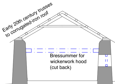
Cross-section at lower end
