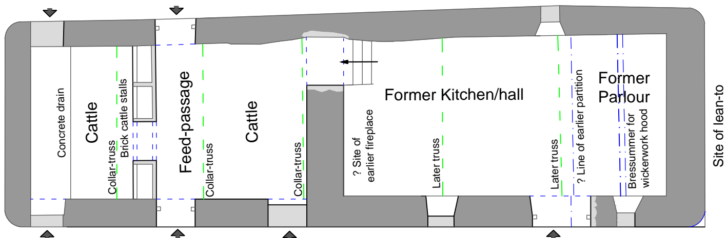
Ground-floor plan
