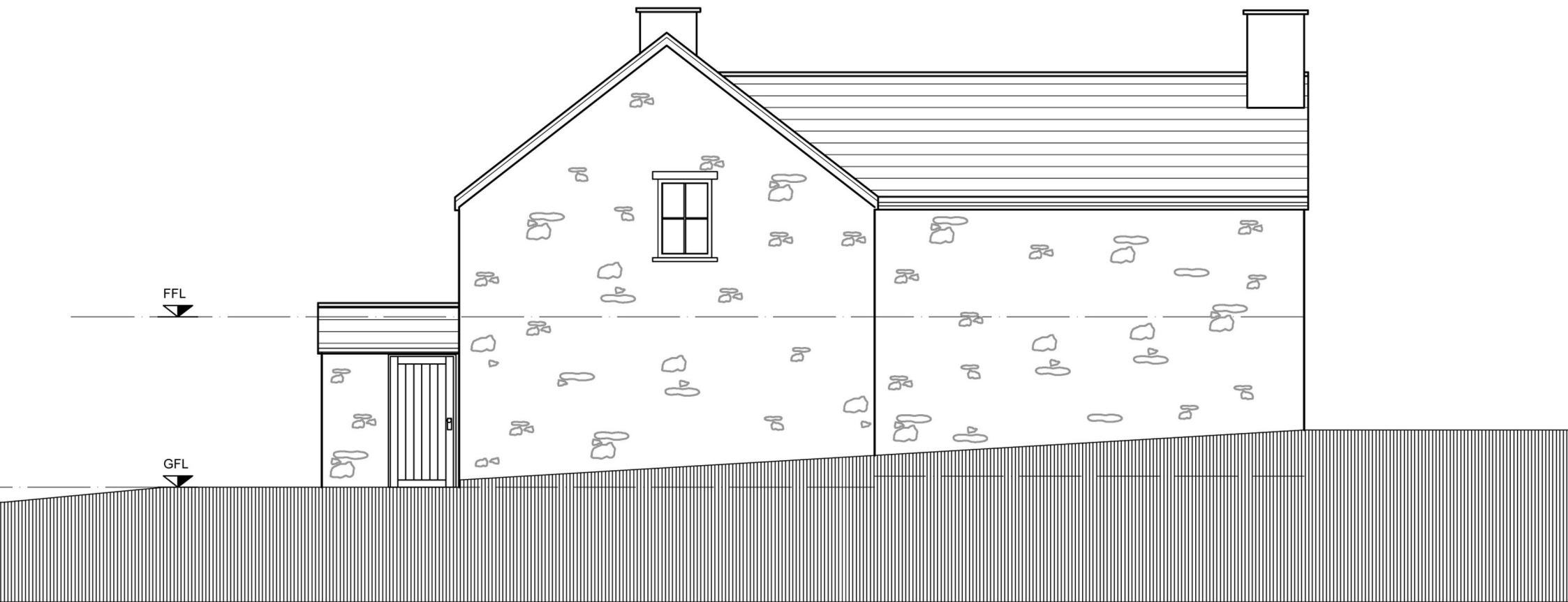
SIDE ELEVATION (SCALE 1:100@A1)
