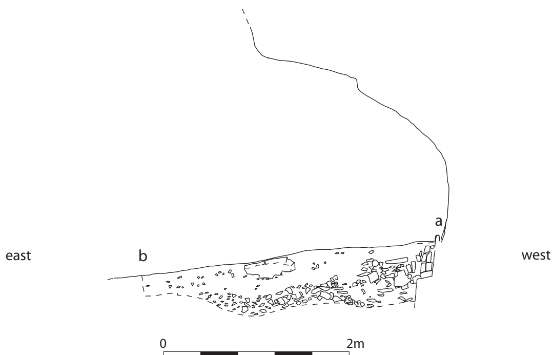
G2179 Snail Cave Fig. 2b : profile of rock shelter in relation to the excavated trench
