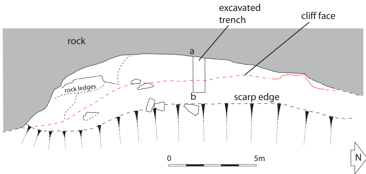
G2179 Snail Cave Fig. 2a : Plan of rock shelter showing location of excavation
