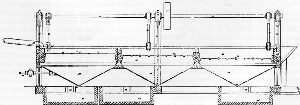
Longitudinal section of Green's Jigger.
