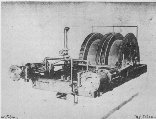
Twin cylinder double acting winding engine sent to Colombia by Greens.
