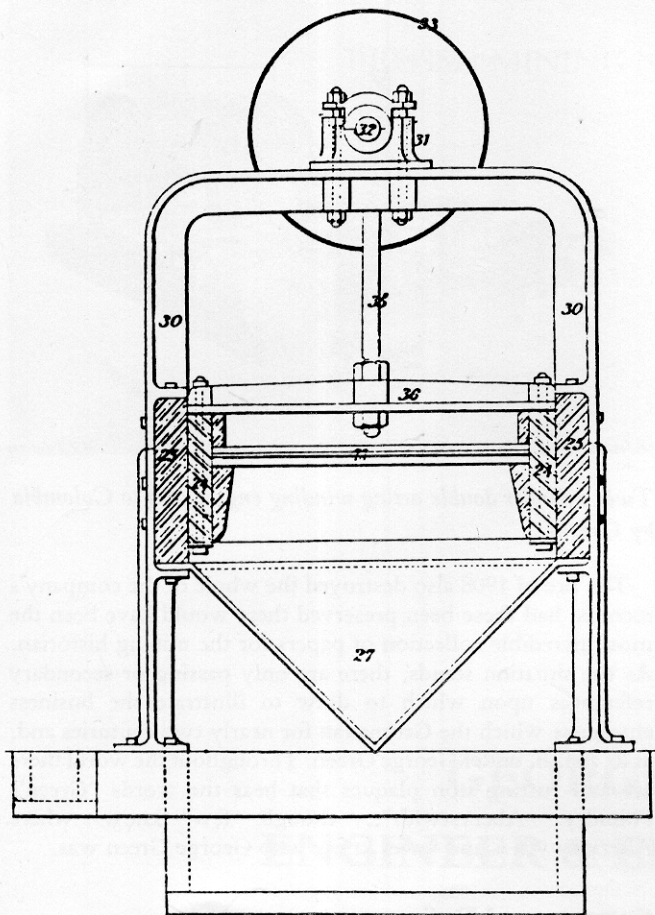
Section of Green's Jigger.
