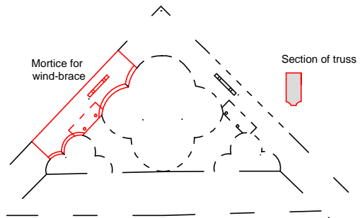
Hall roof truss reconstruction from re-used lintel (shown in red)
