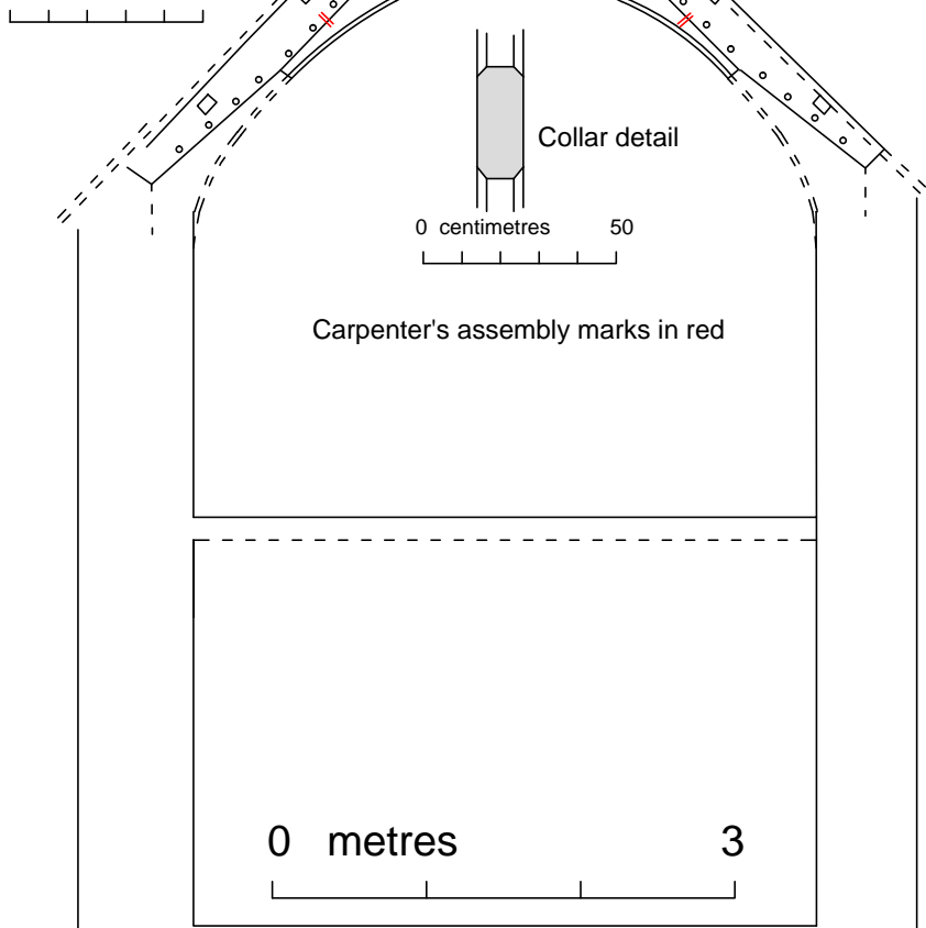
Cross-section of chapel roof
