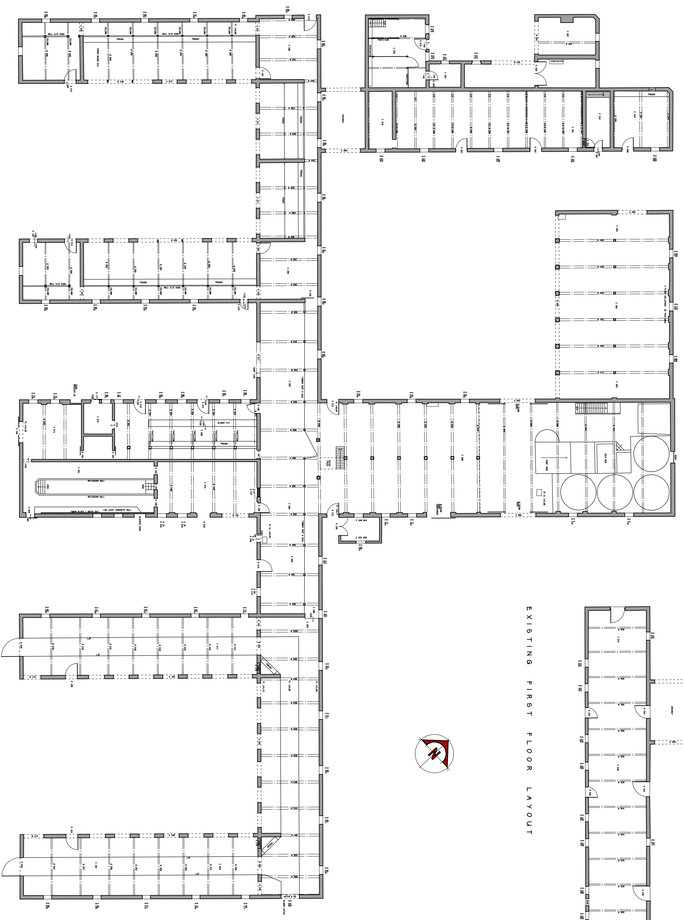
EXISTING GROUND FLOOR LAYOUT
