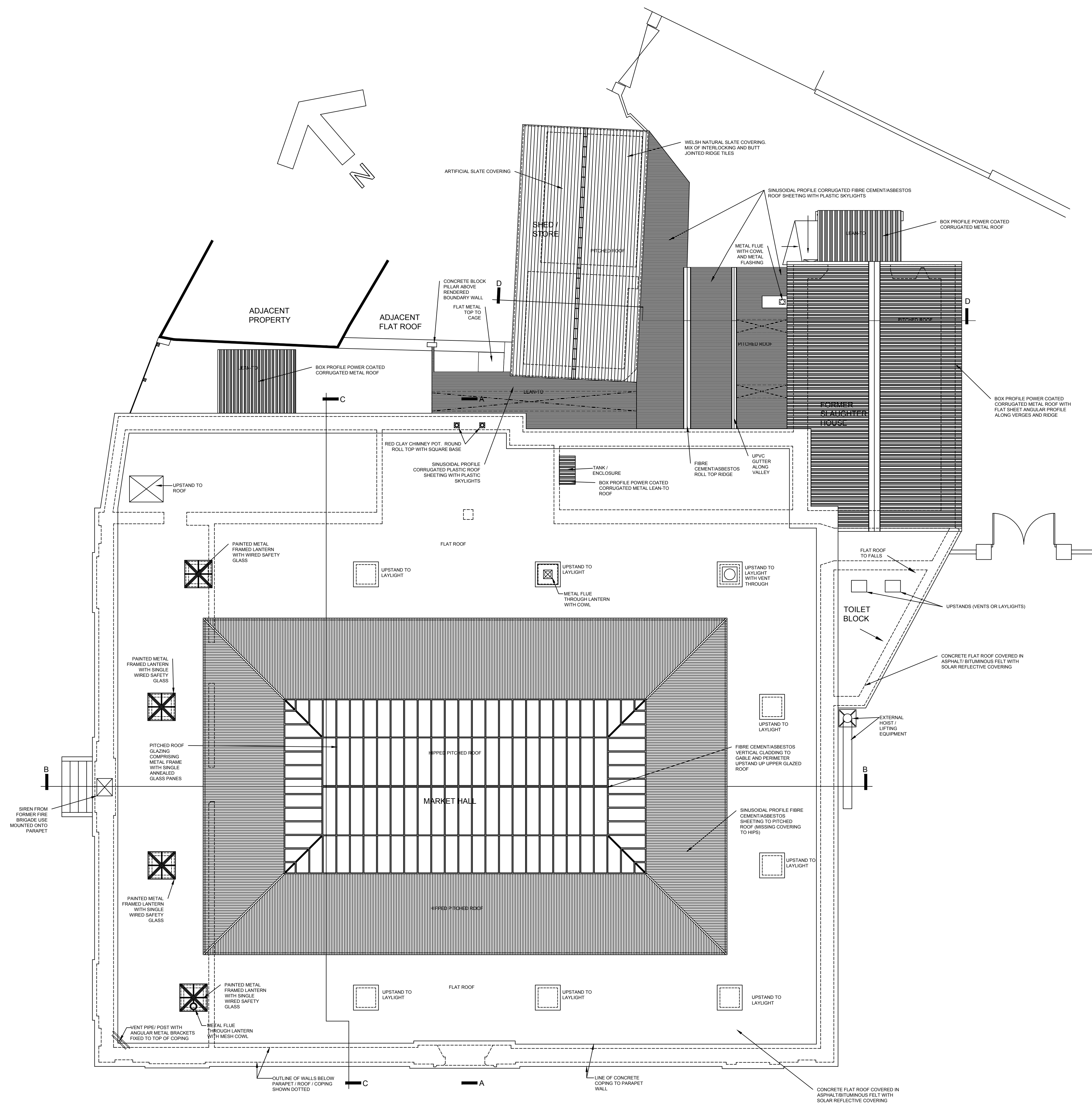
EXISTING ROOF PLAN 1:100
