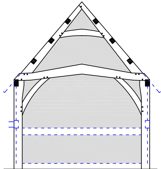
Hall closed truss at lower south end
