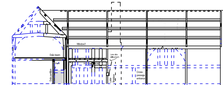
Hall central arch-braced truss
