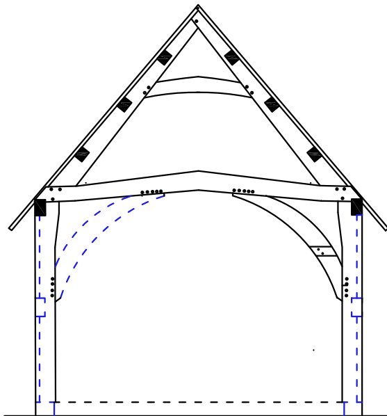
Hall central arch-braced truss
