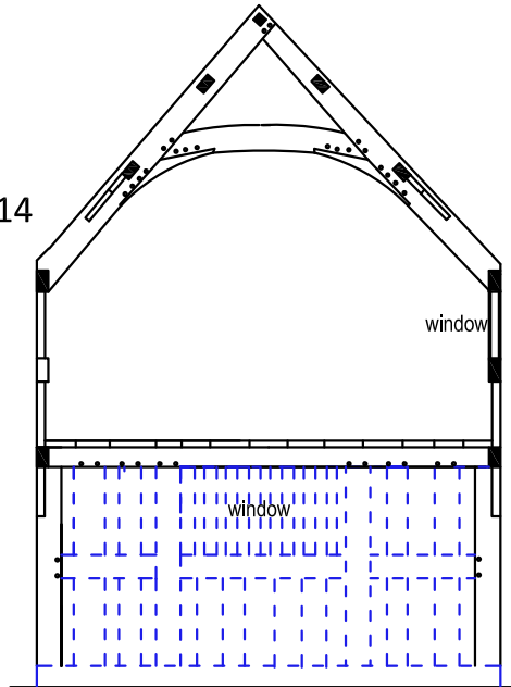
Cross-wing section through open-bay
