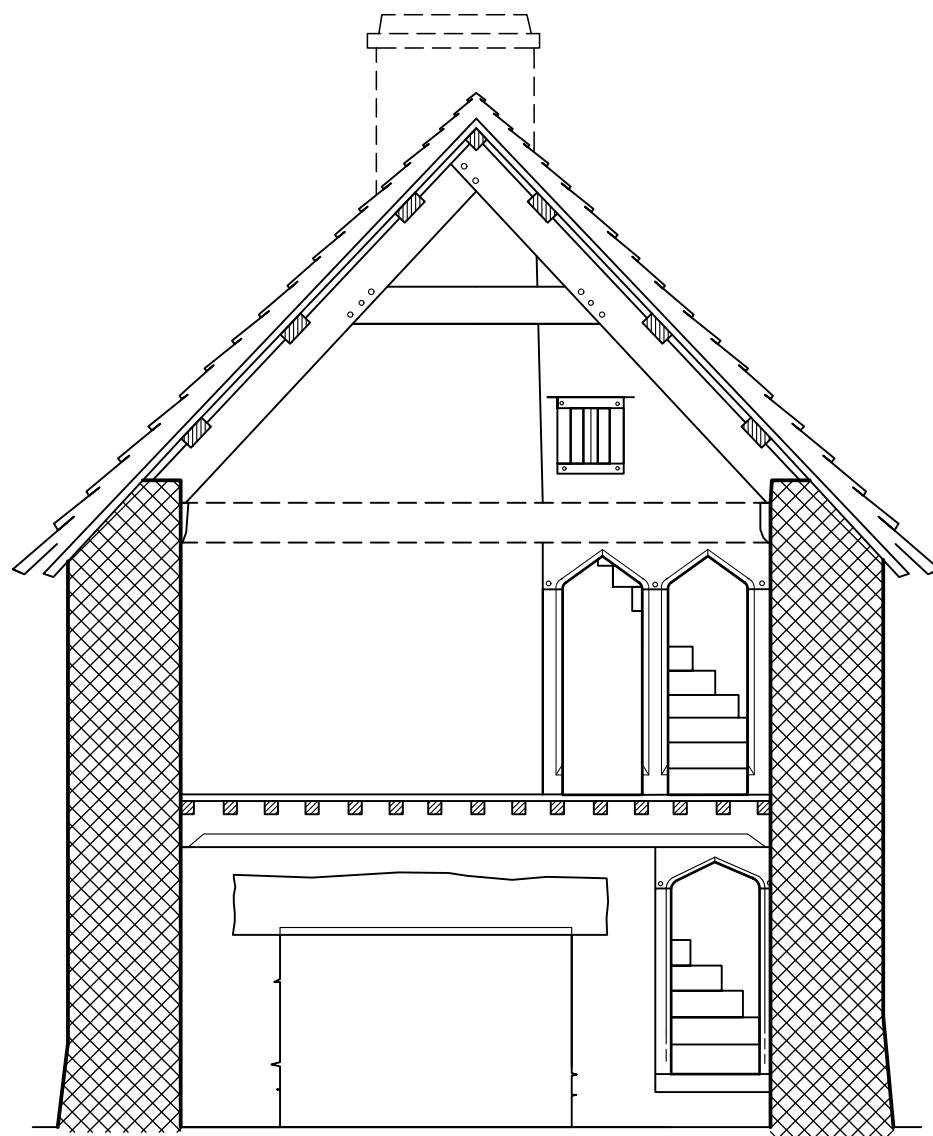
Cross-section through hall
