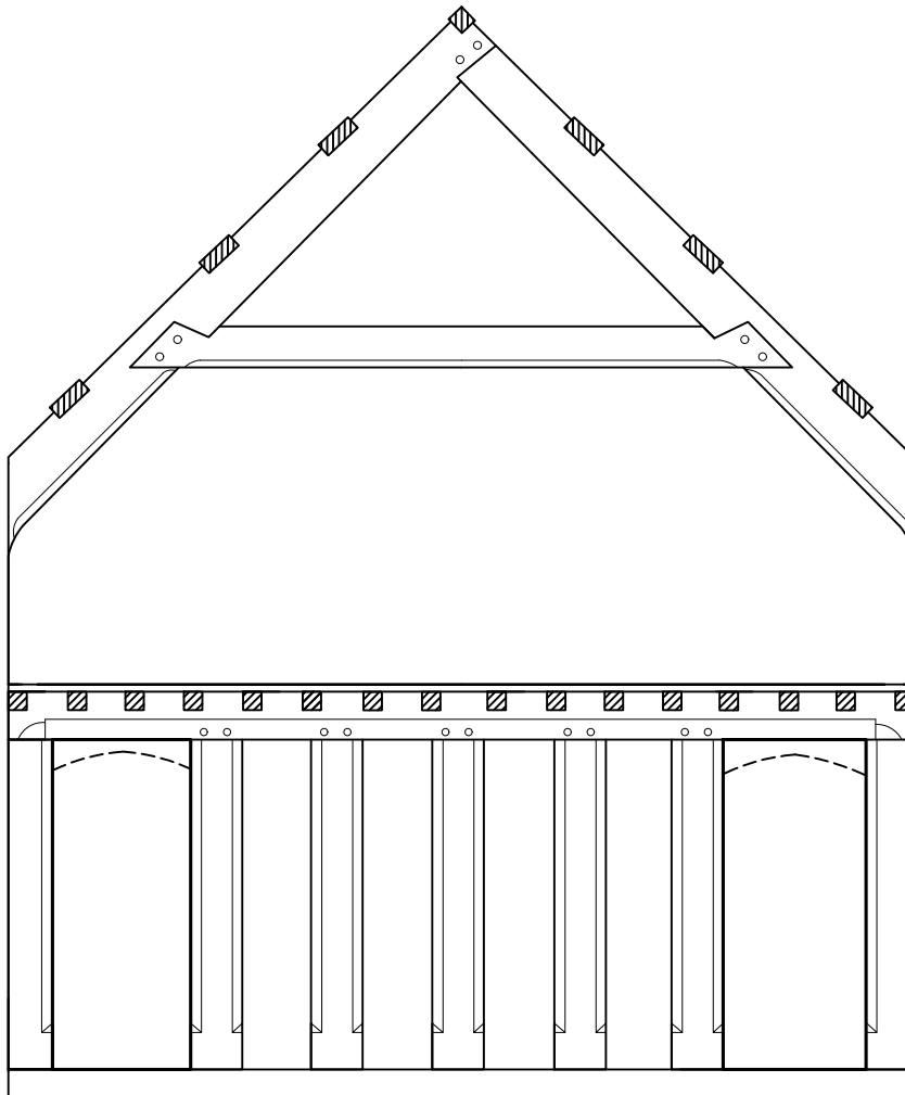
Roof truss & partition, Park Cottage
