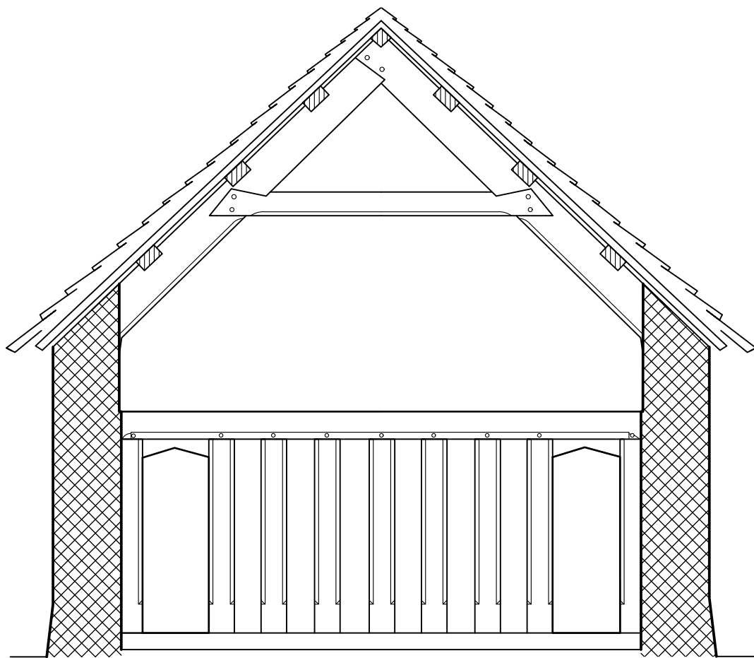
Cross section of hall
