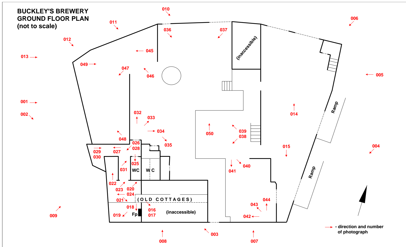
Figure 2: Brewery building, ground floor plan and photographic key
