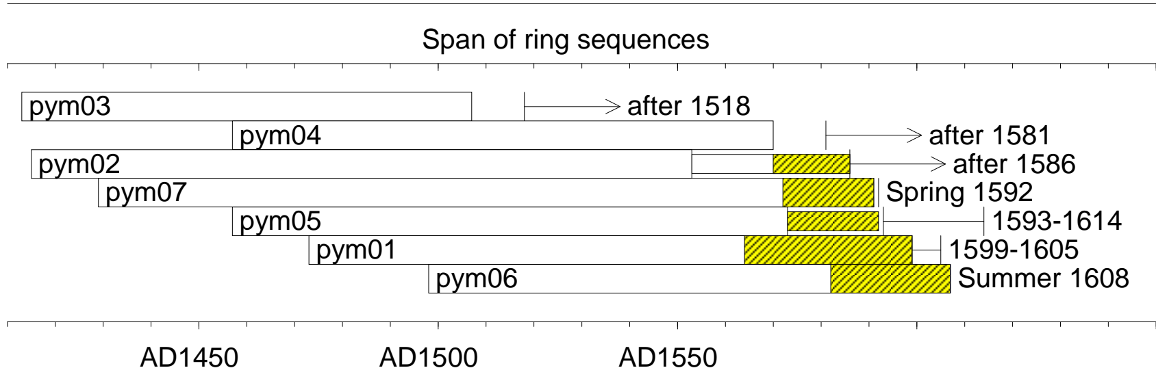
Figure 2: Bar diagram showing the relative positions of overlap of the dated series, along with their interpreted likely, or actual, felling date ranges. Hatched yellow sections represent sapwood rings, and narrow sections of bar represent additional unmeasured rings
