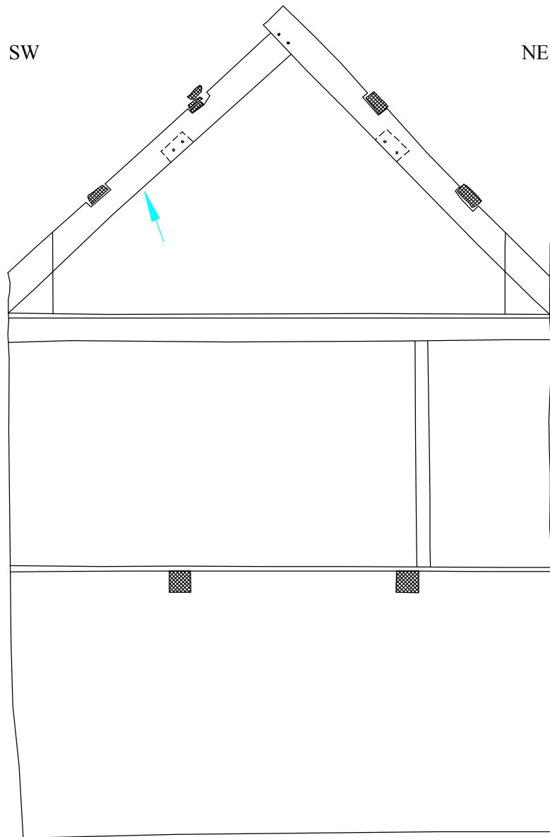
Figure 7: Truss 1 Scale 1:50
