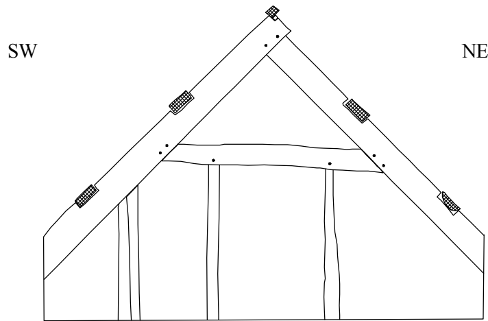
8.1: Truss 2
