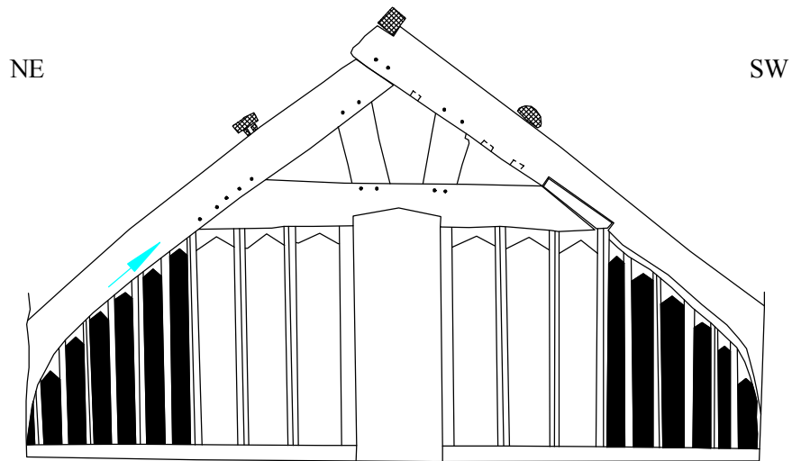
8.2: Truss 3
