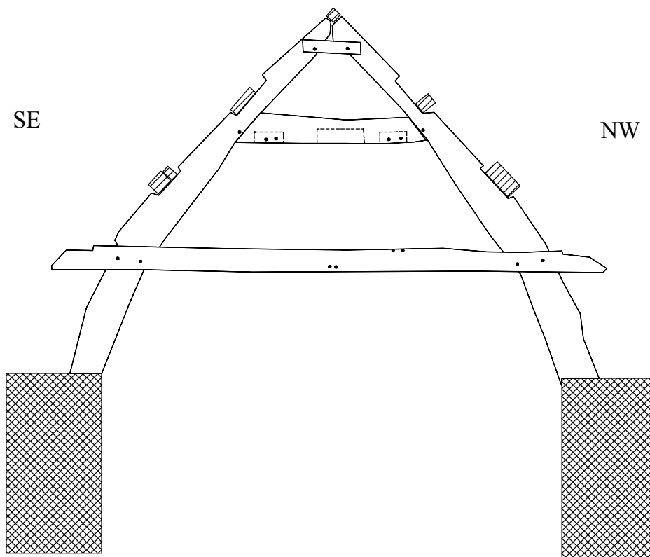
Truss 1
