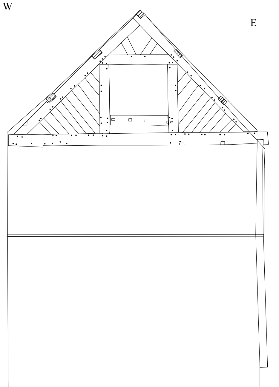
Main Range Truss 3
