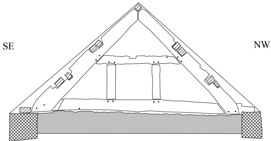
Gable End Truss
